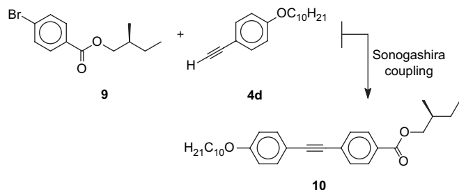
Scheme 4. Synthesis of 10 .
